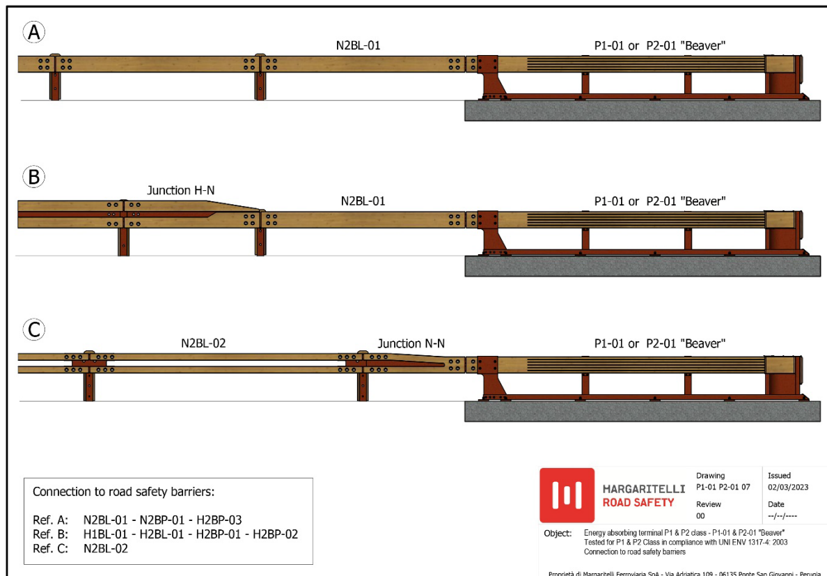
Figure 11 Connection with P1-01 and P2-01 Beaver terminals
