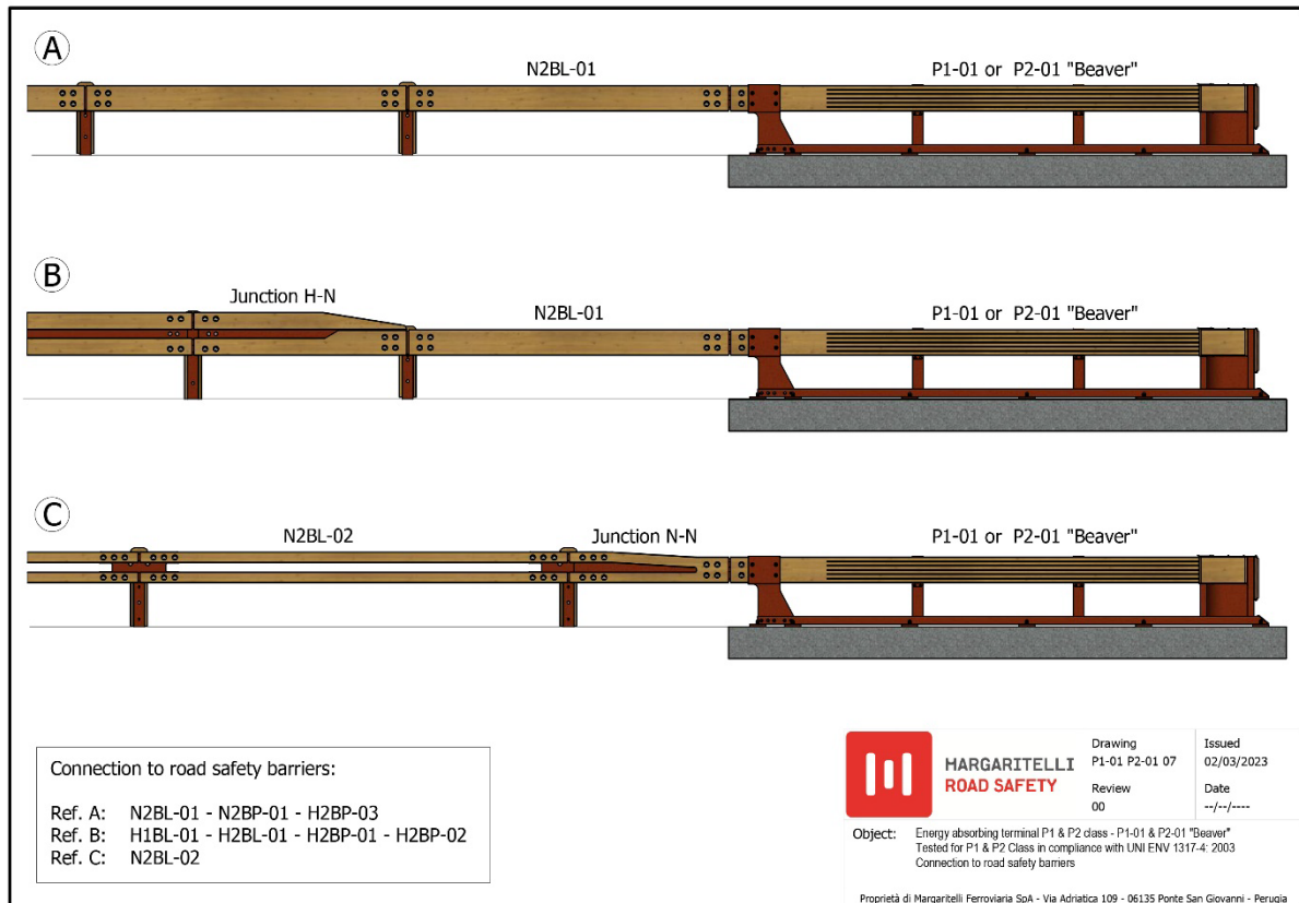
Figure 9 Connection with P1-01 and P2-01 Beaver terminals
