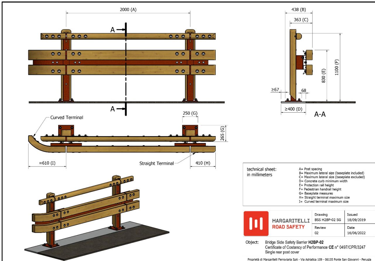
Figure 5 H2BP-02 barrier in standard version
