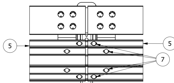
Step "B" - Corrugated splice plate & protection rail assembly
