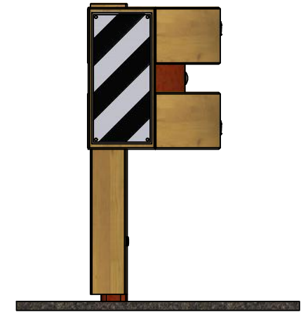
Front view with panel
