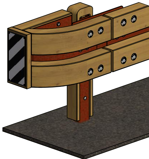
T50-01 with panel
